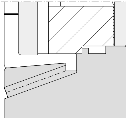
Paneelvak (P)
